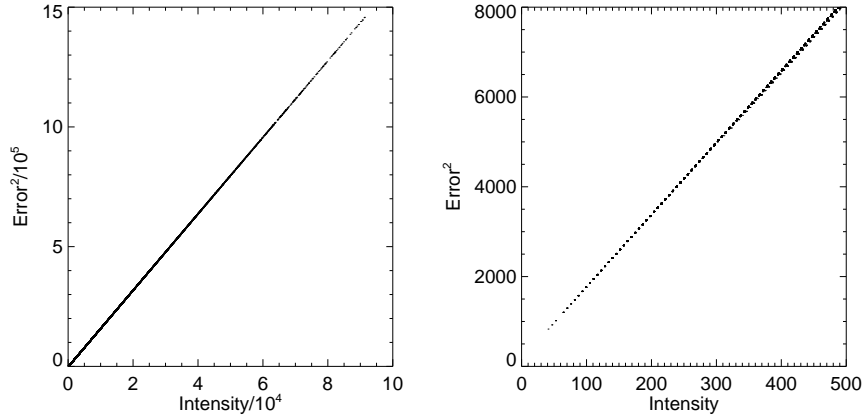
Figure 2: Plots of error squared versus intensity for the Fe XII \lambda 195.12 data window of the 2006 December 2 10:33 data-set. The left panel shows all the data points; the right panel shows the values for low intensities.
