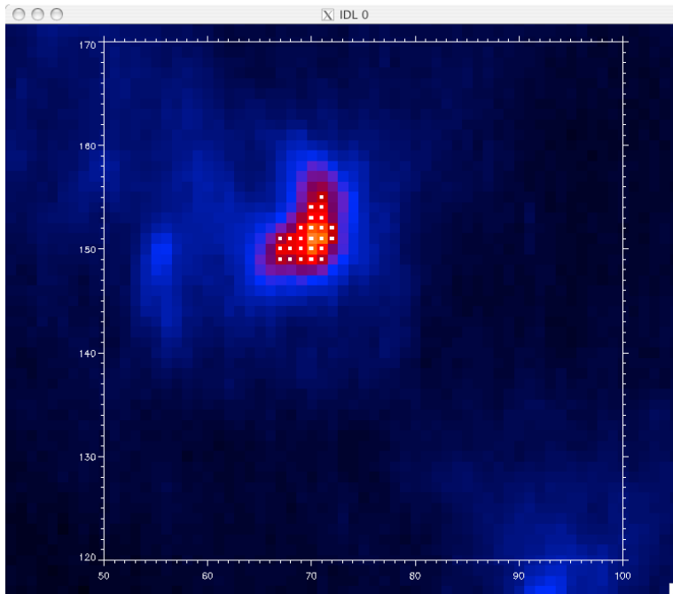
Figure 2. Fe VIII image showing the selected pixels (small white squares).
